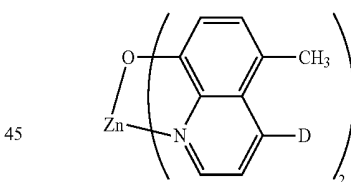
[Chemical Formula 4-1]
