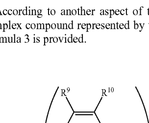
[Chemical Formula 3]
