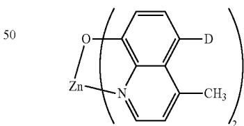
[Chemical Formula 4-2]
